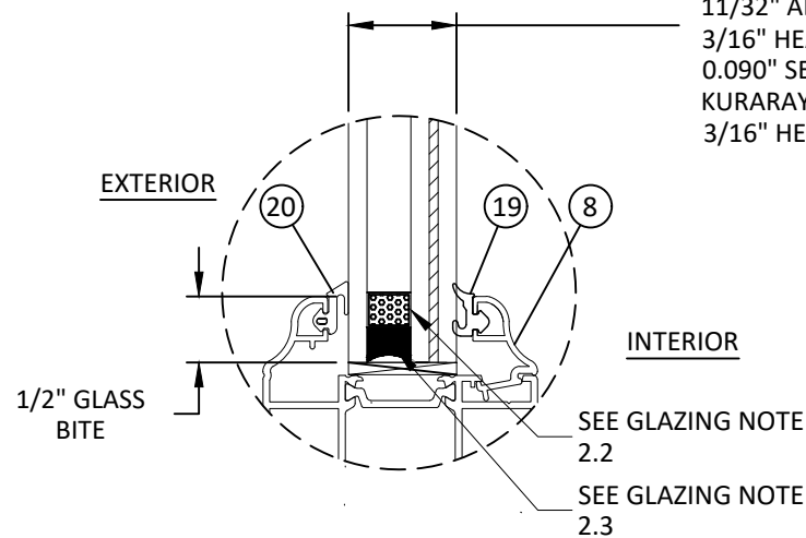
GLAZING DETAIL 1
