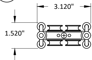
26 END CARRIER SET ALUMINUM 6063-T5
