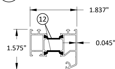
42 PANNEL RAIL ALUMINUM 6063-T5
