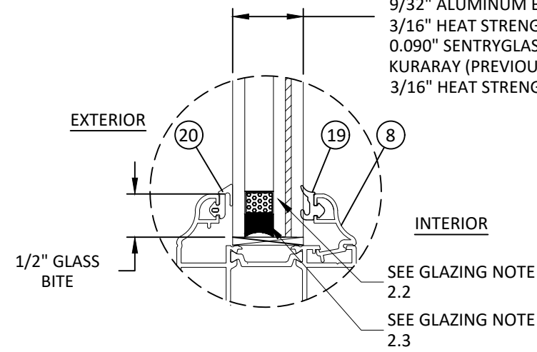
GLAZING DETAIL 2
