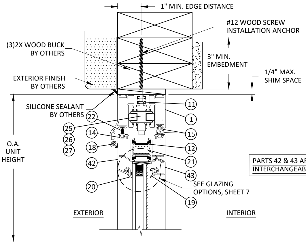
B 5 VERTICAL SECTION HEAD - 2X WOOD BUCK
