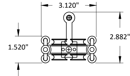
25 INTERMEDIATE CARRIER SET ALUMINUM 6063-T5
