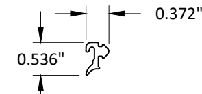
19 INTERIOR GLAZING GASKET EPDM
