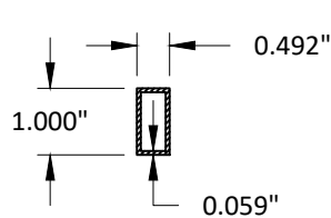
21 REINFORCEMENT ALUMINUM 6063-T5
