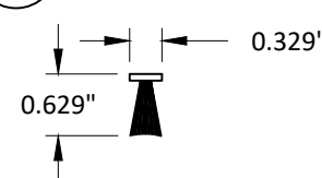
41 BOTTOM PILE POLYETHYLENE
