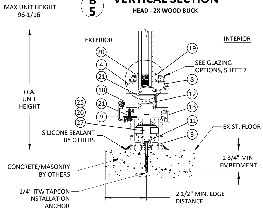
A 5 VERTICAL SECTION SILL - CONCRETE/MASONRY WATER BARRIER THRESHOLD
