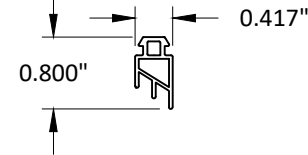
13 BOTTOM RAIL GASKET EPDM
