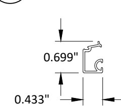
43 GLAZING BEAD ALUMINUM 6063-T5
